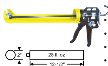
59-155 Caulking Applicator
