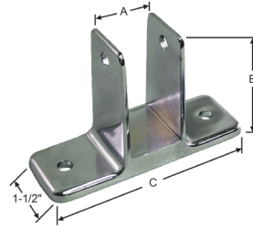
Two Ears Wall Brackets
