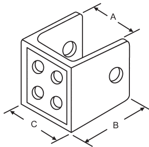
U- Brackets
