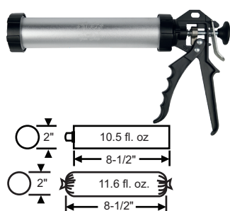
59-159 Aluminium Barrel Applicator HPS400-A
