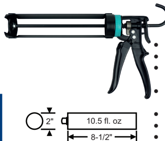
59-105 Half Pipe Caulking Applicator FX7-90
